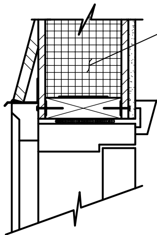
TYPICAL HEADER DETAIL
