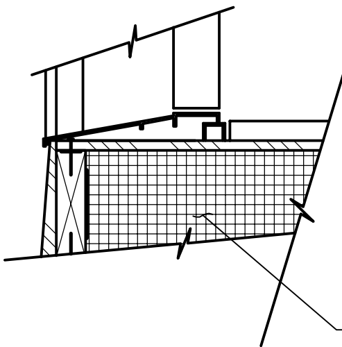
TYPICAL EXTERIOR SILL DETAIL
