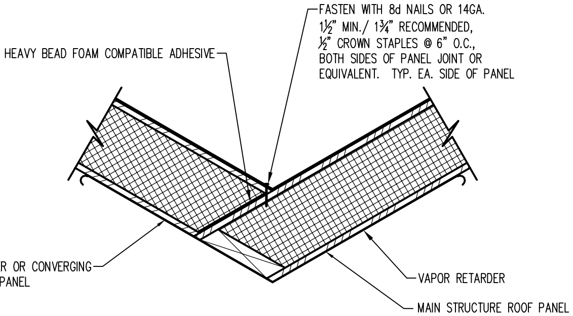
SECTION THROUGH ALTERNATE VALLEY
